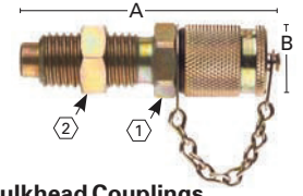
Bulkhead Couplings
