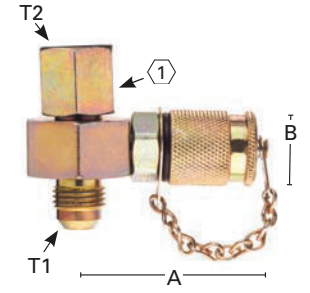
Swivel Run Tee with Test Coupling
